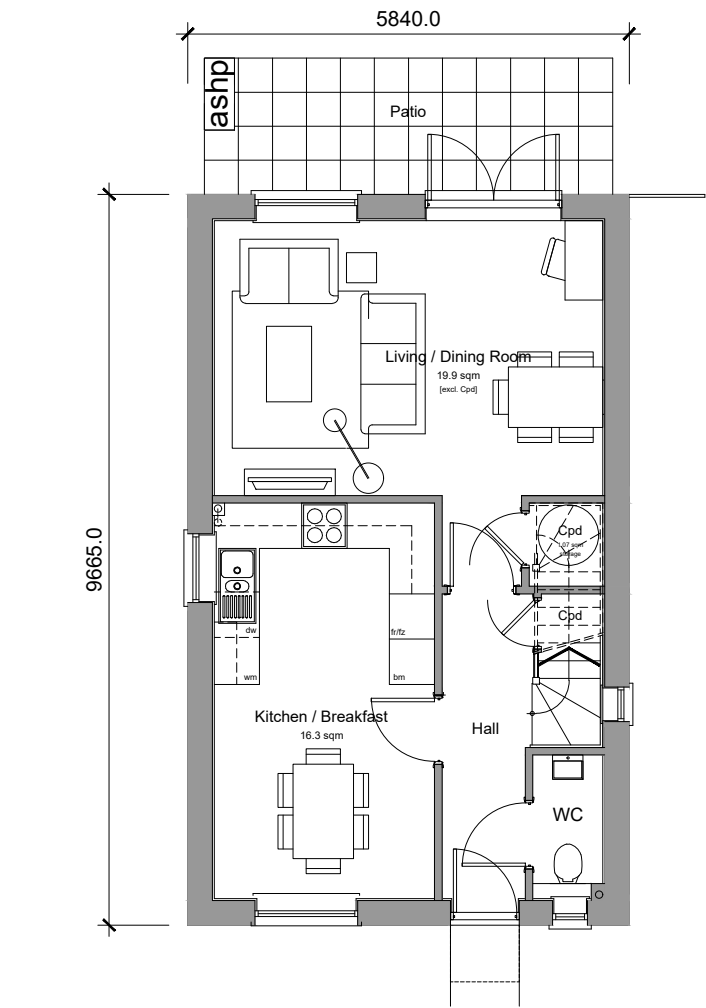
Ground Floor Plan 3-Bedroom 4-Person House 92.16sqm / 990sqft GIA (to finishes)
