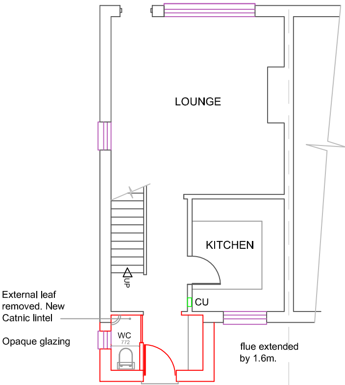
GROUND FLOOR PLAN PROPOSED
