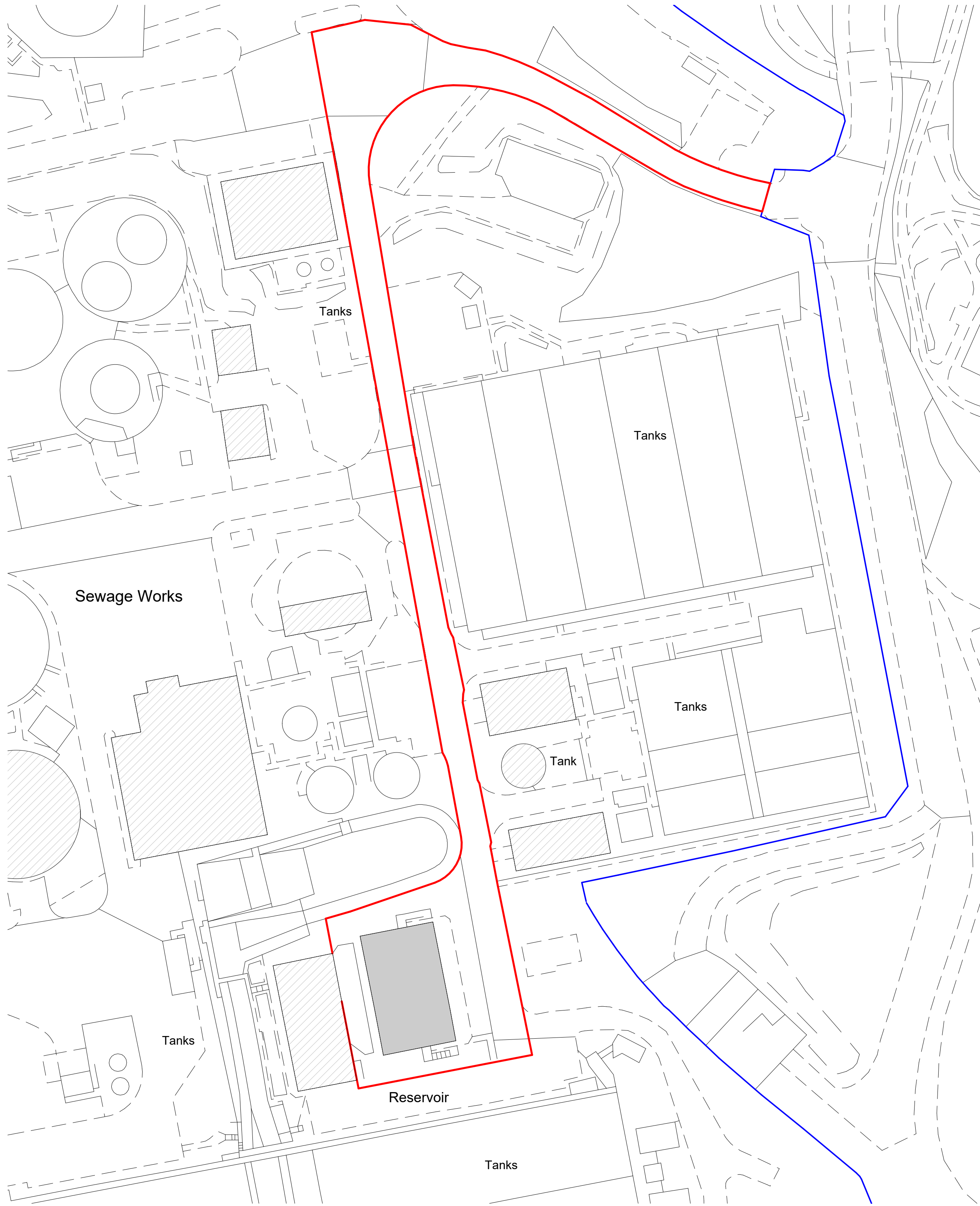
2 Block Plan 1 : 500 0m 10m 20m 30m 40m 50m VISUAL SCALE 1:500 @ A1
