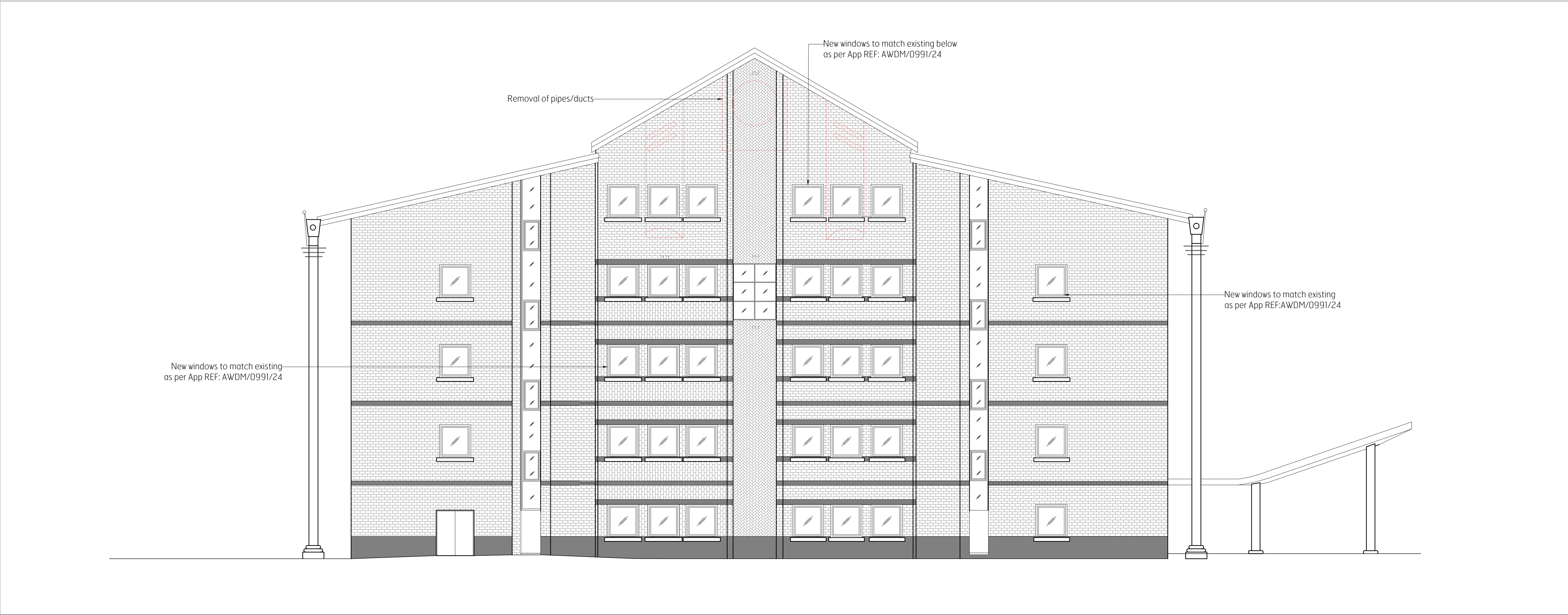
Proposed West (side) Elevation 1:100@A1
