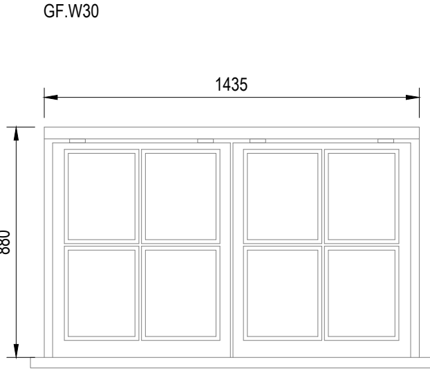
EXISTING EXTERNAL ELEVATION
