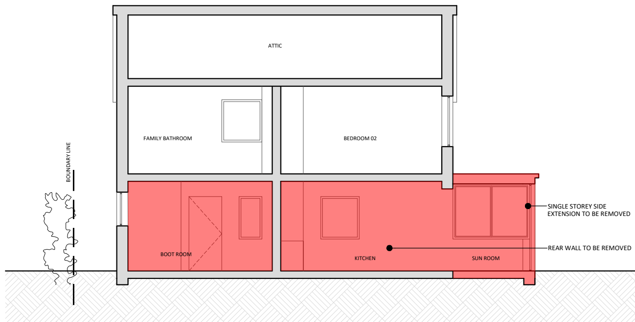
2 EXISTING SECTION B-B SCALE 1:100
