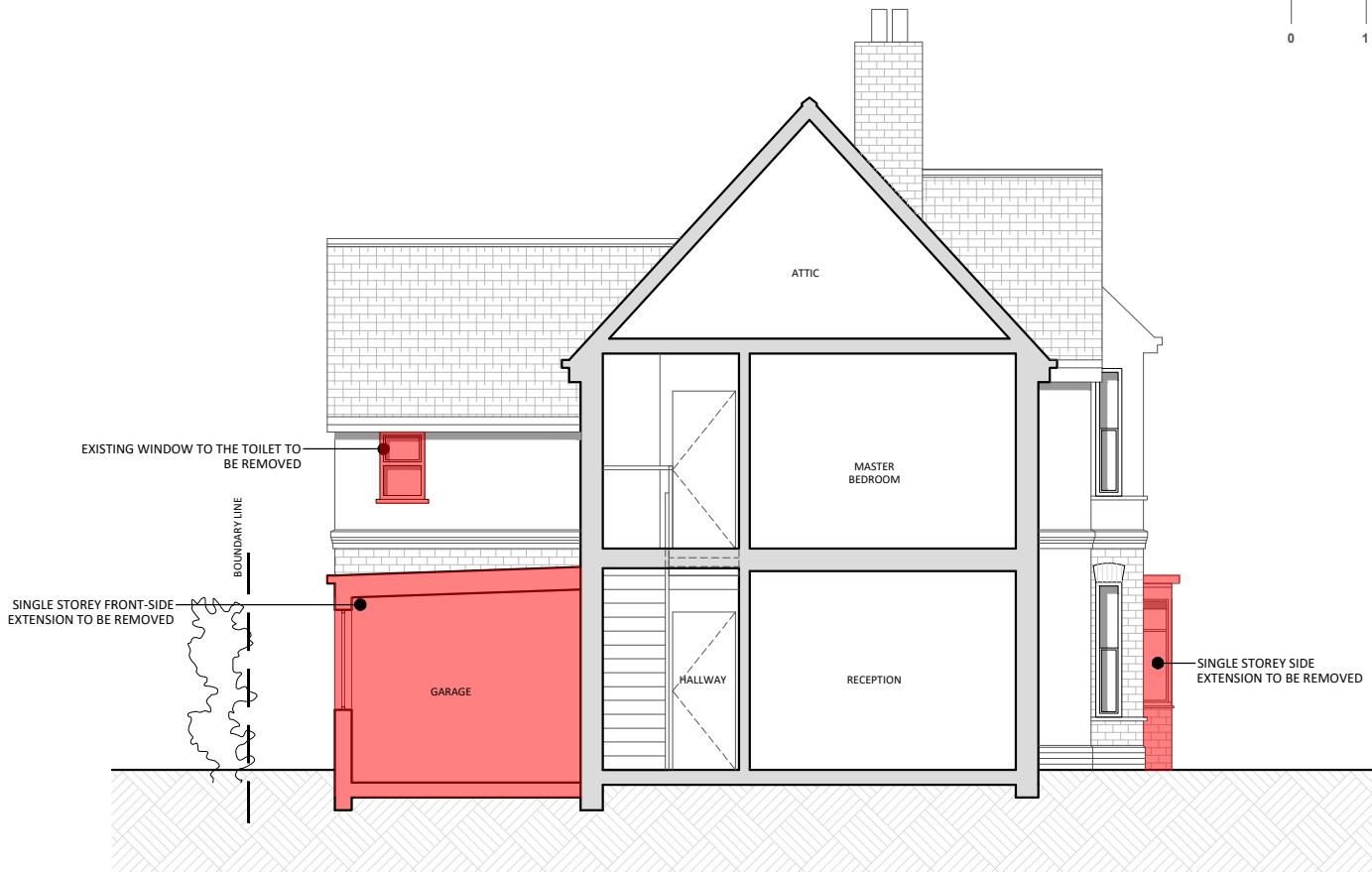
1 EXISTING SECTION A-A SCALE 1:100
