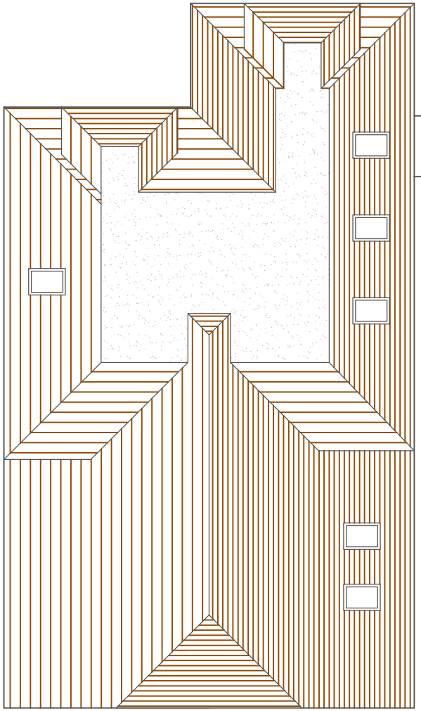
ROOF PLAN EXISTING
