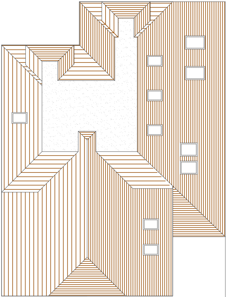
ROOF PLAN PROPOSED
