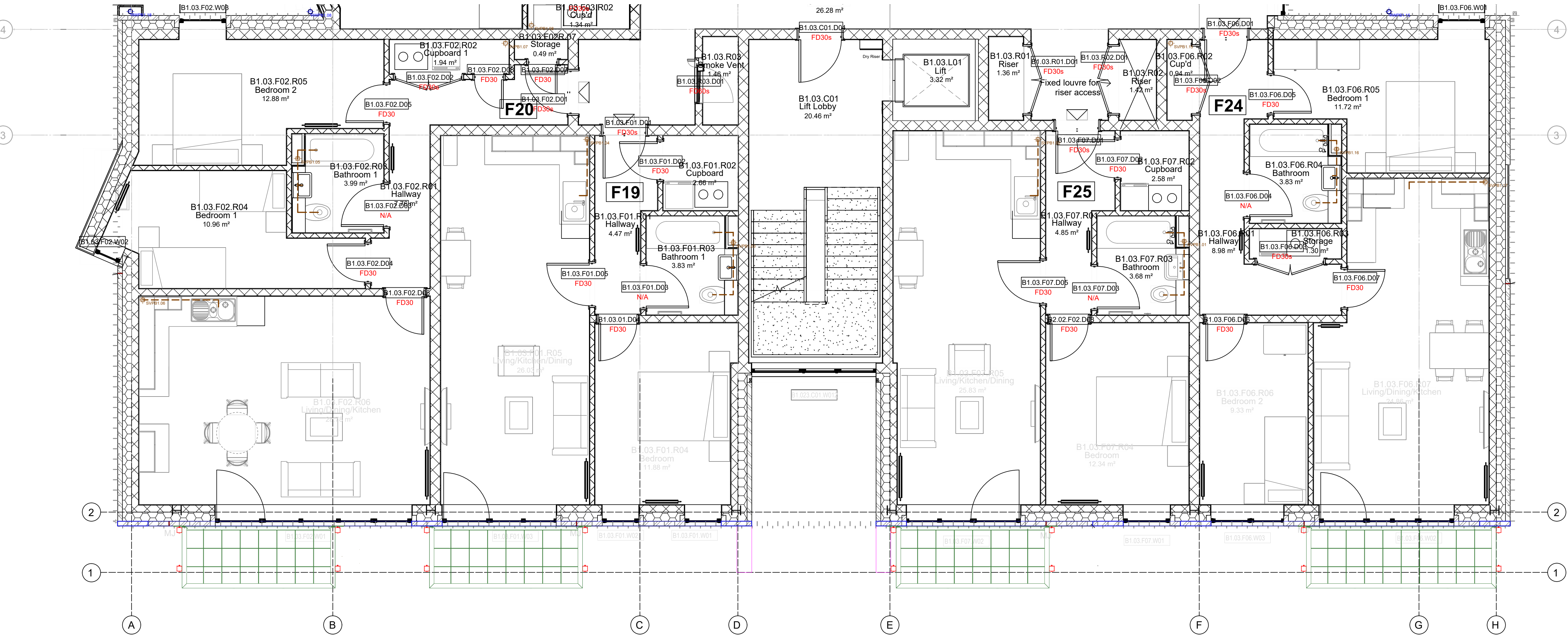
BUILDING 1 THIRD FLOOR GA PLAN 1:50 SCALE @ A1
