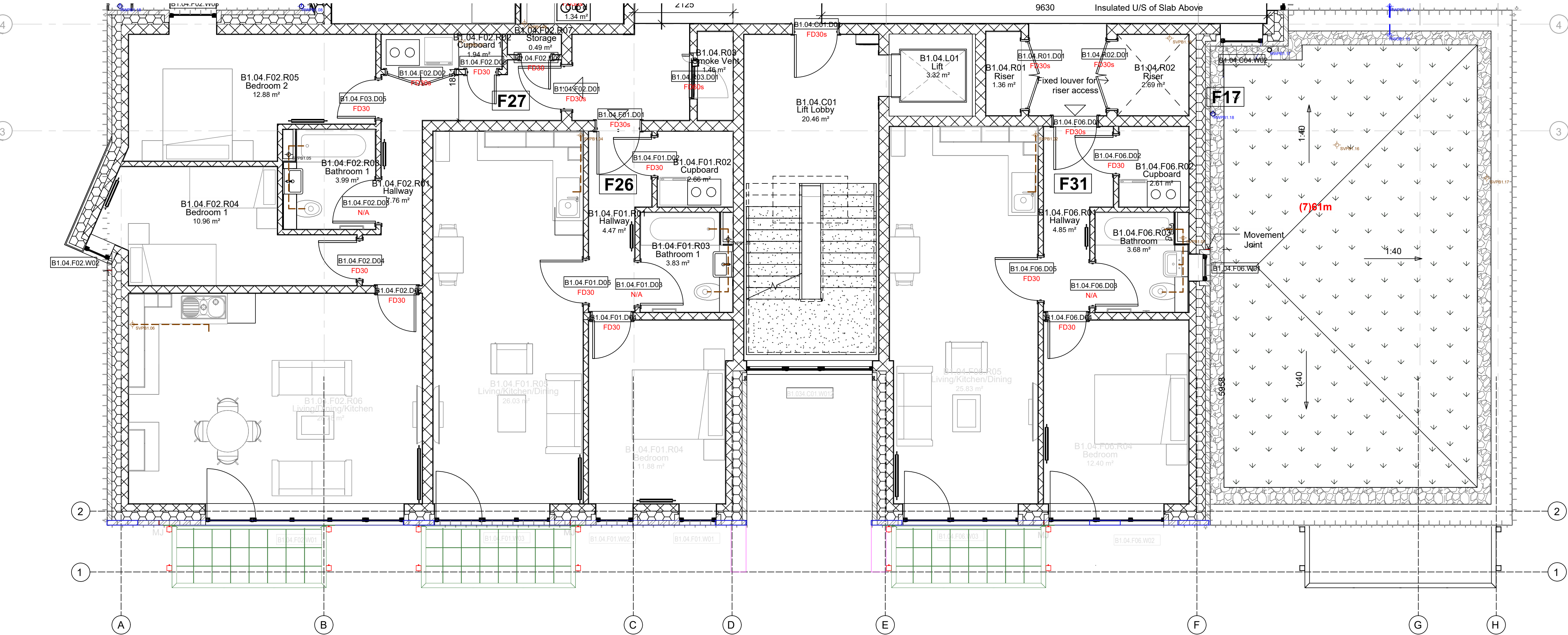
BUILDING 1 FOURTH FLOOR GA PART PLAN 1:50 SCALE @ A1
