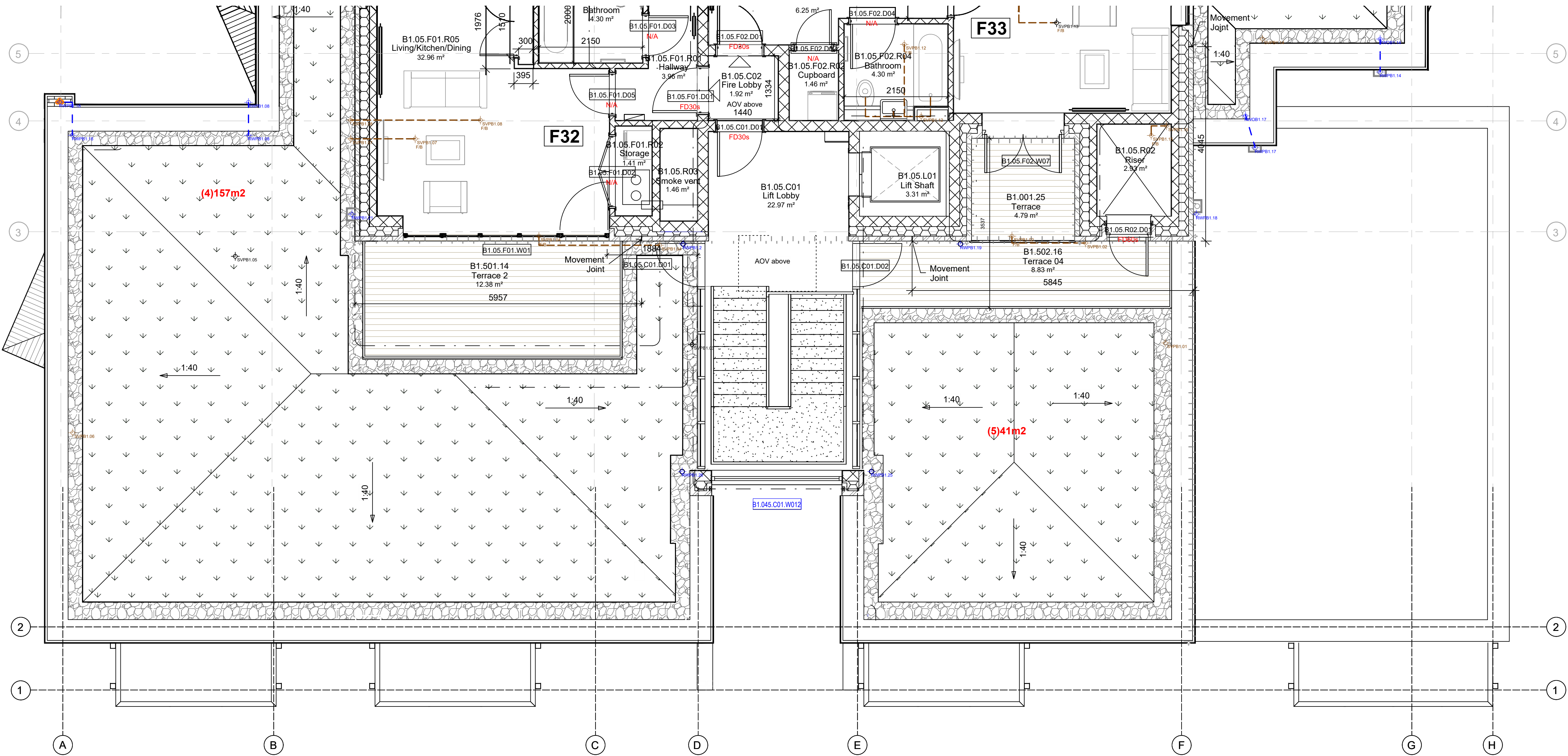
BUILDING 1 FIFTH FLOOR PART GA PLAN 1:50 SCALE @ A1
