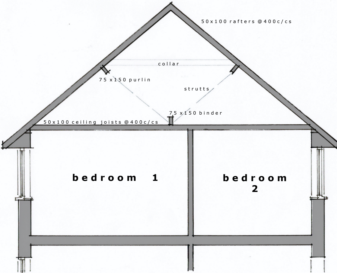
SECTION 1:50
