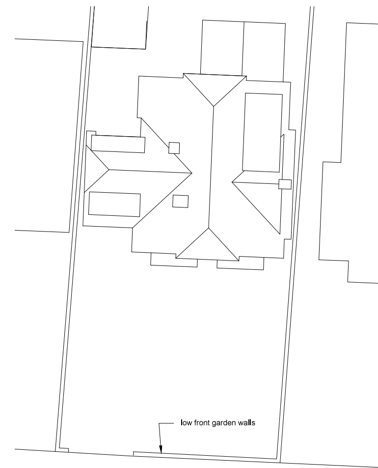
030.3 PRE-EXISTING FRONT GARDEN PLAN scale 1:200
