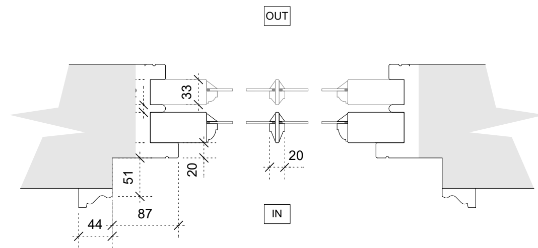
WINDOW TYPE - EW04 TIMBER SASH PUTTY EXTERNALLY HORIZONTAL SECTION 1:5 @ A3
