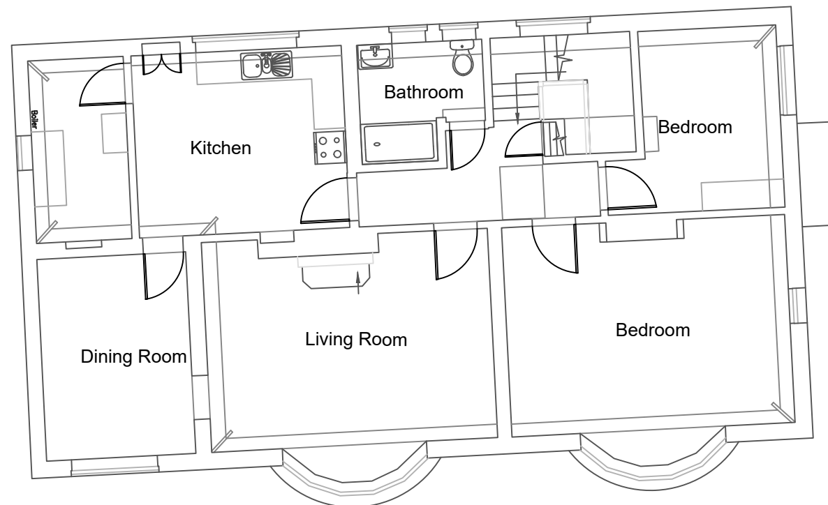
EXISTING FIRST FLOOR PLAN 1:100 @ A3
