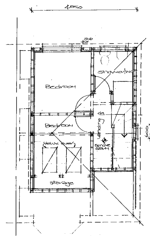
Proposed Second Floor Plan scale 1/100
