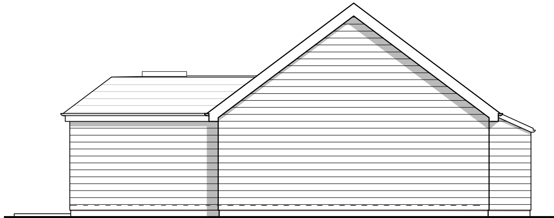
04 SIDE (NORTH) ELEVATION D.02 AS PROPOSED_1:100 @ A3
