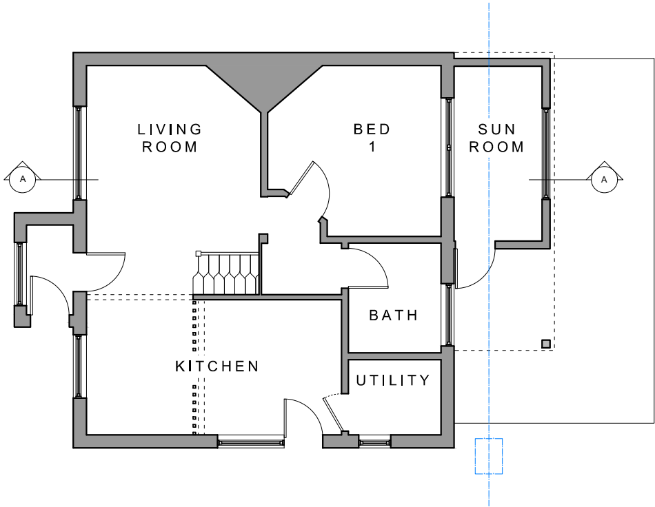
01 S.01 GROUND FLOOR PLAN AS EXISTING_1:100 @ A3
