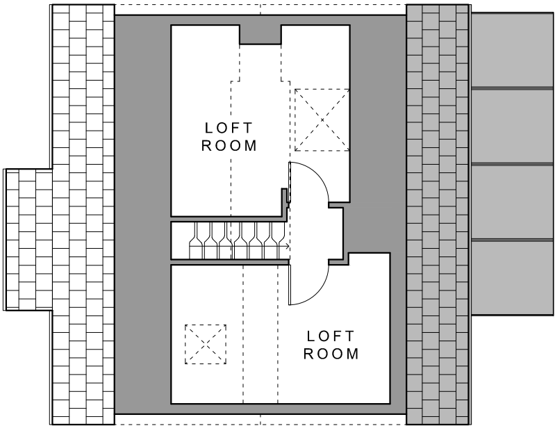
02 S.01 FIRST FLOOR PLAN AS EXISTING_1:100 @ A3
