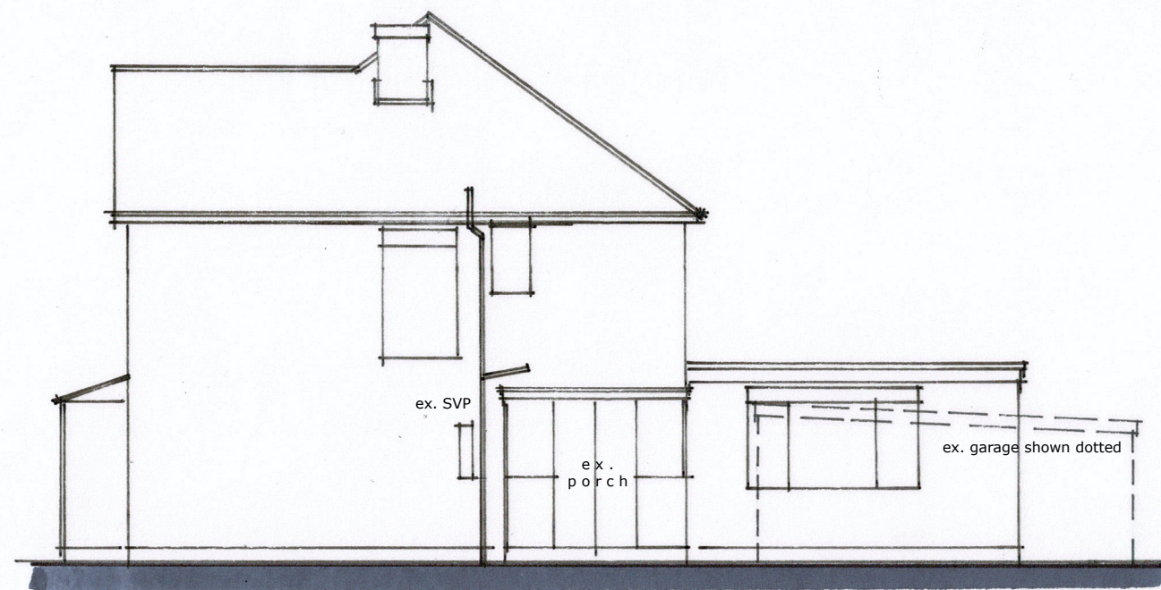
SIDE (e) ELEVATION 1:100 @ A3
