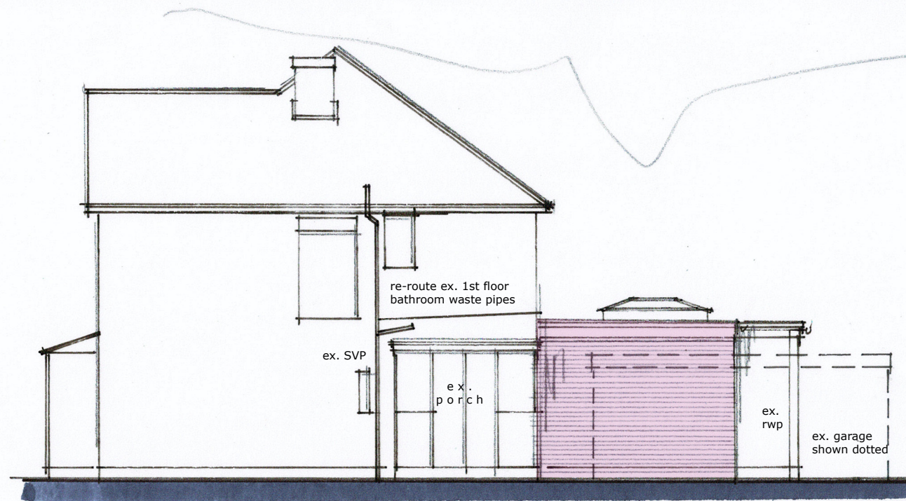
SIDE (e) ELEVATION 1:100 @ A3
