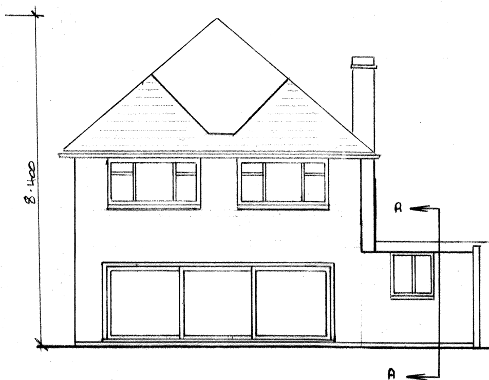
PROPOSED REAR ELEVATION (NORTH)
