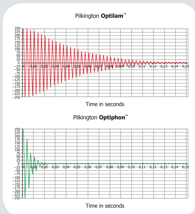
Figure 9: The illustration shows the impressive damping differences between Pilkington Optilam ™ and Pilkington Optiphon ™ from the sound engineering point of view.
