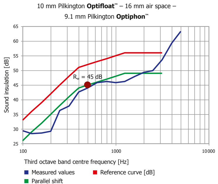
Figure 4: Determining the sound insulation value R_w
