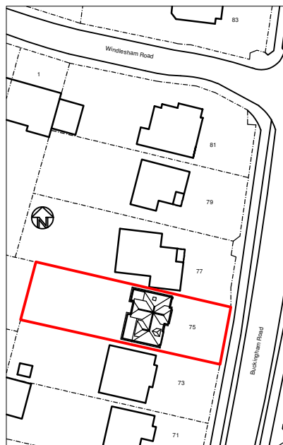
Location Plan 1:250
