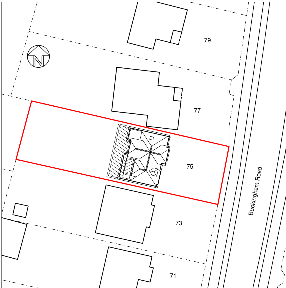
Block Plan 1:500
