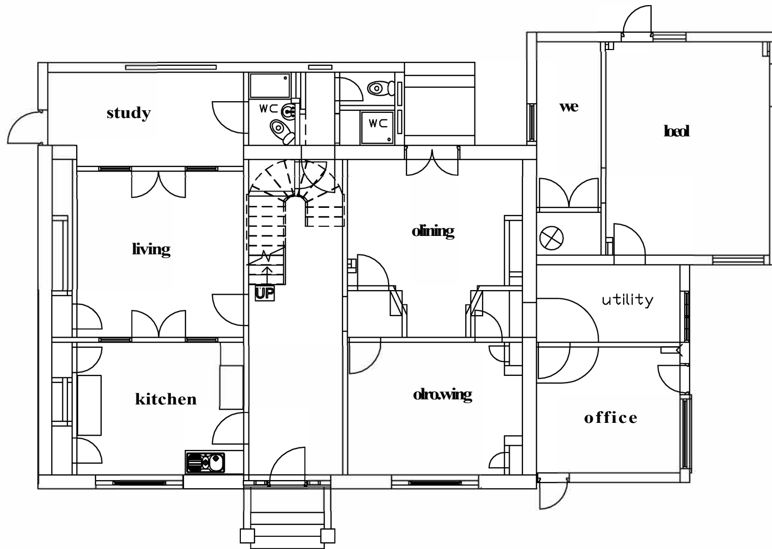
ground floor
