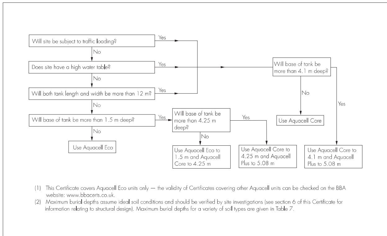
Figure 2 Sustainable drainage system selection and design
