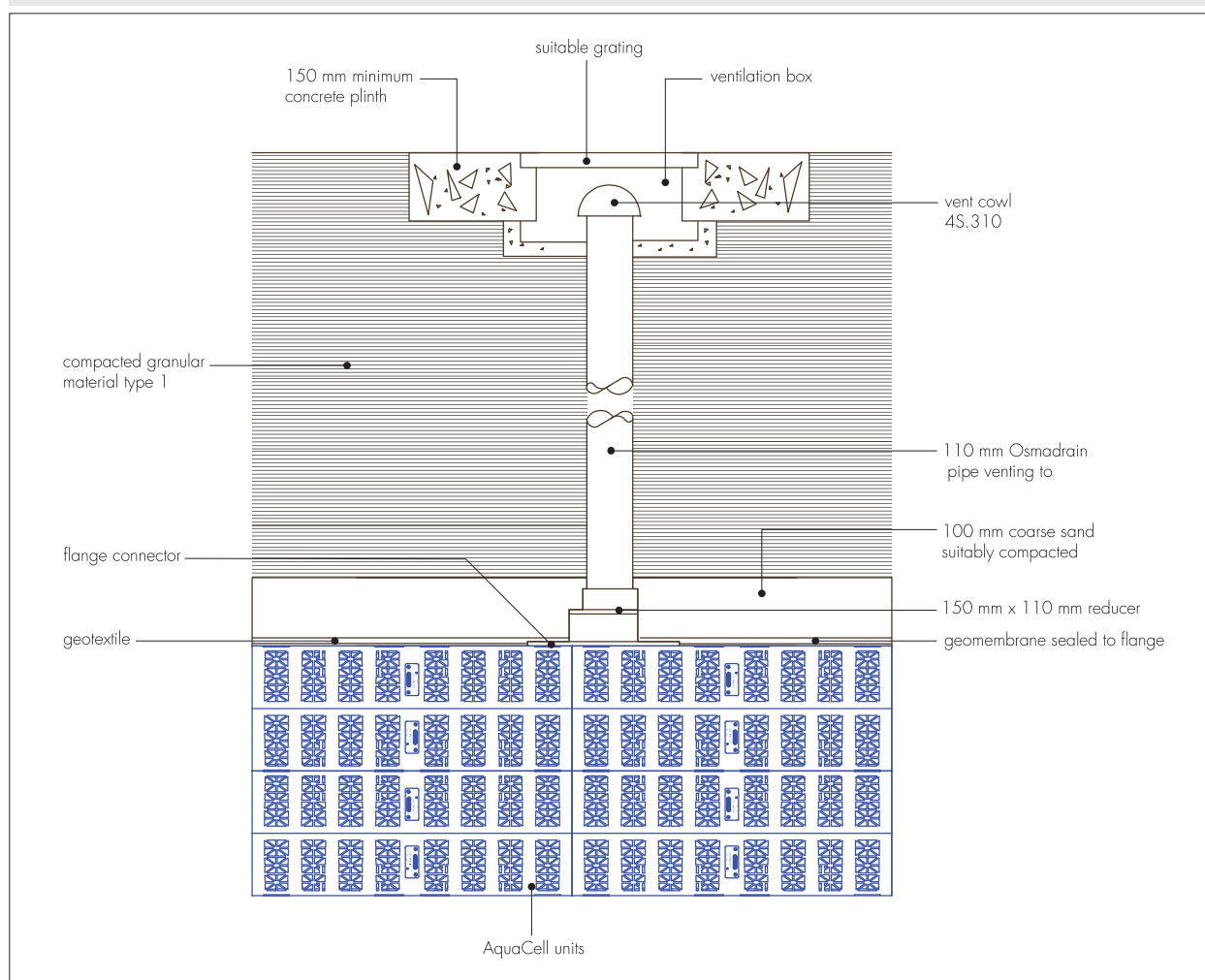
Figure 4 Typical air vent system
