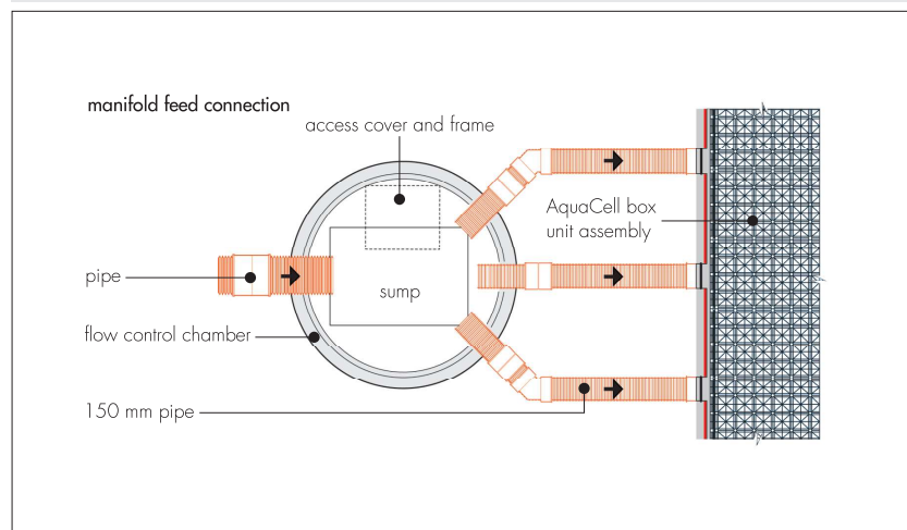
Figure 3 Typical inlet connection design
