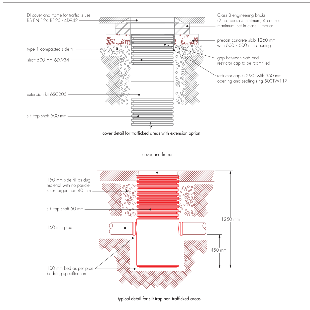
Figure 5 Typical silt trap
