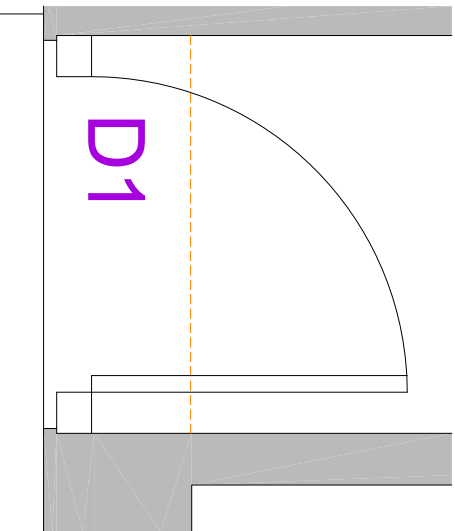
Proposed Plan Section @ 1 : 20
