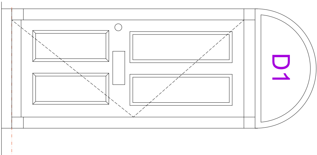
Proposed Elevation @ 1 : 20
