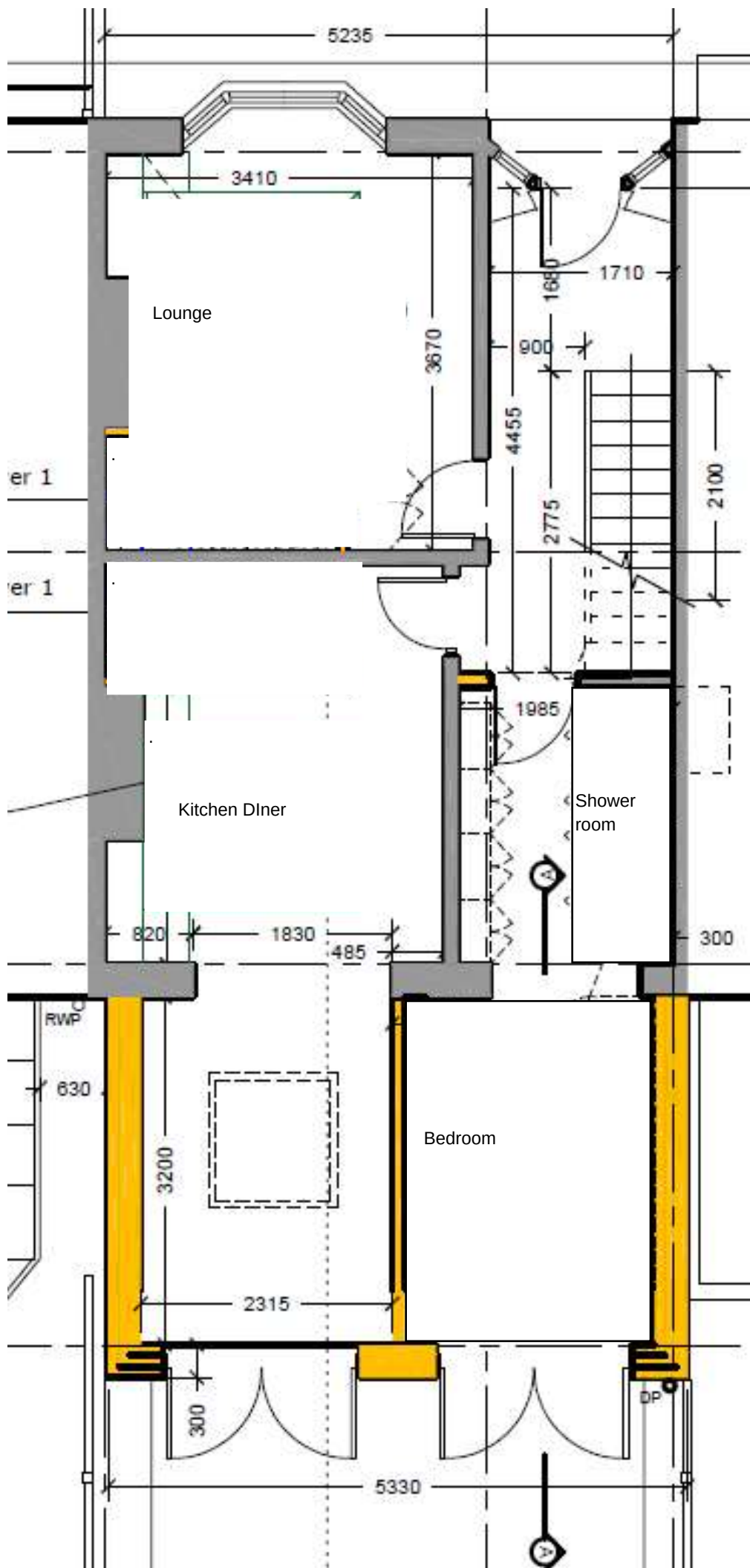
Ground floor existing floor plan
