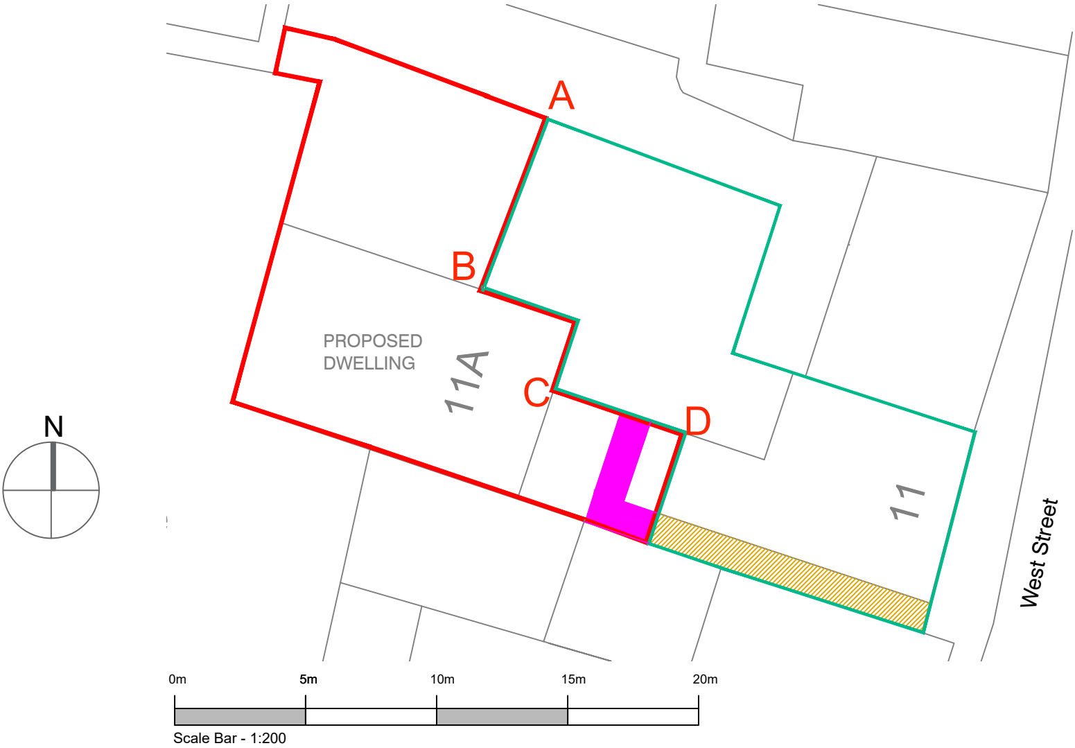
BLOCK PLAN 1:200
