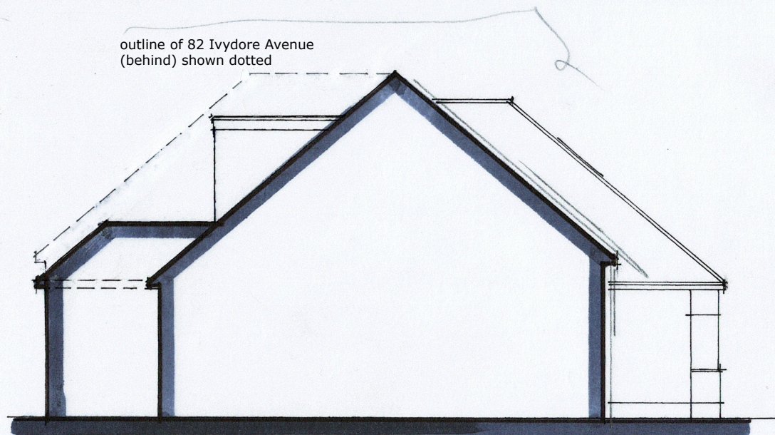
SIDE (n) ELEVATION 1:100 @ A3
