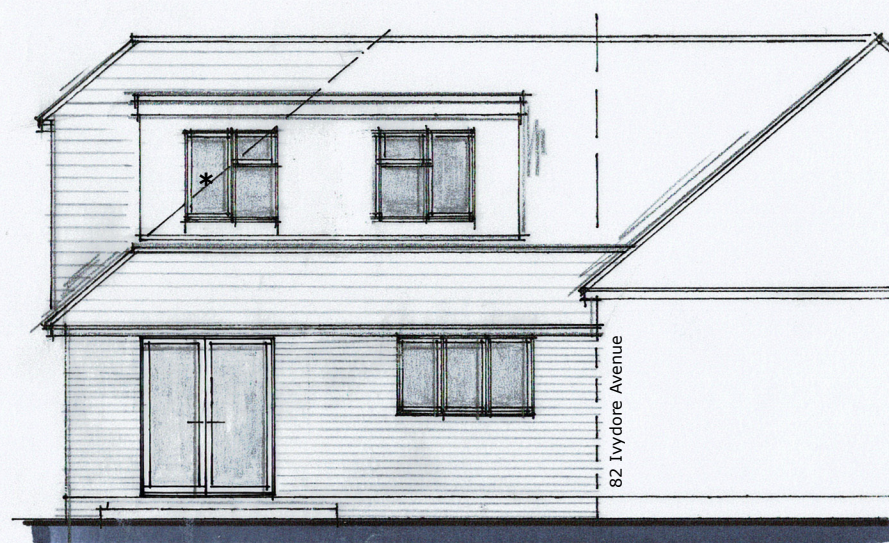
SIDE (e)
