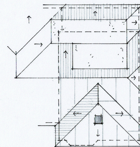
ROOF PLAN 1:200
