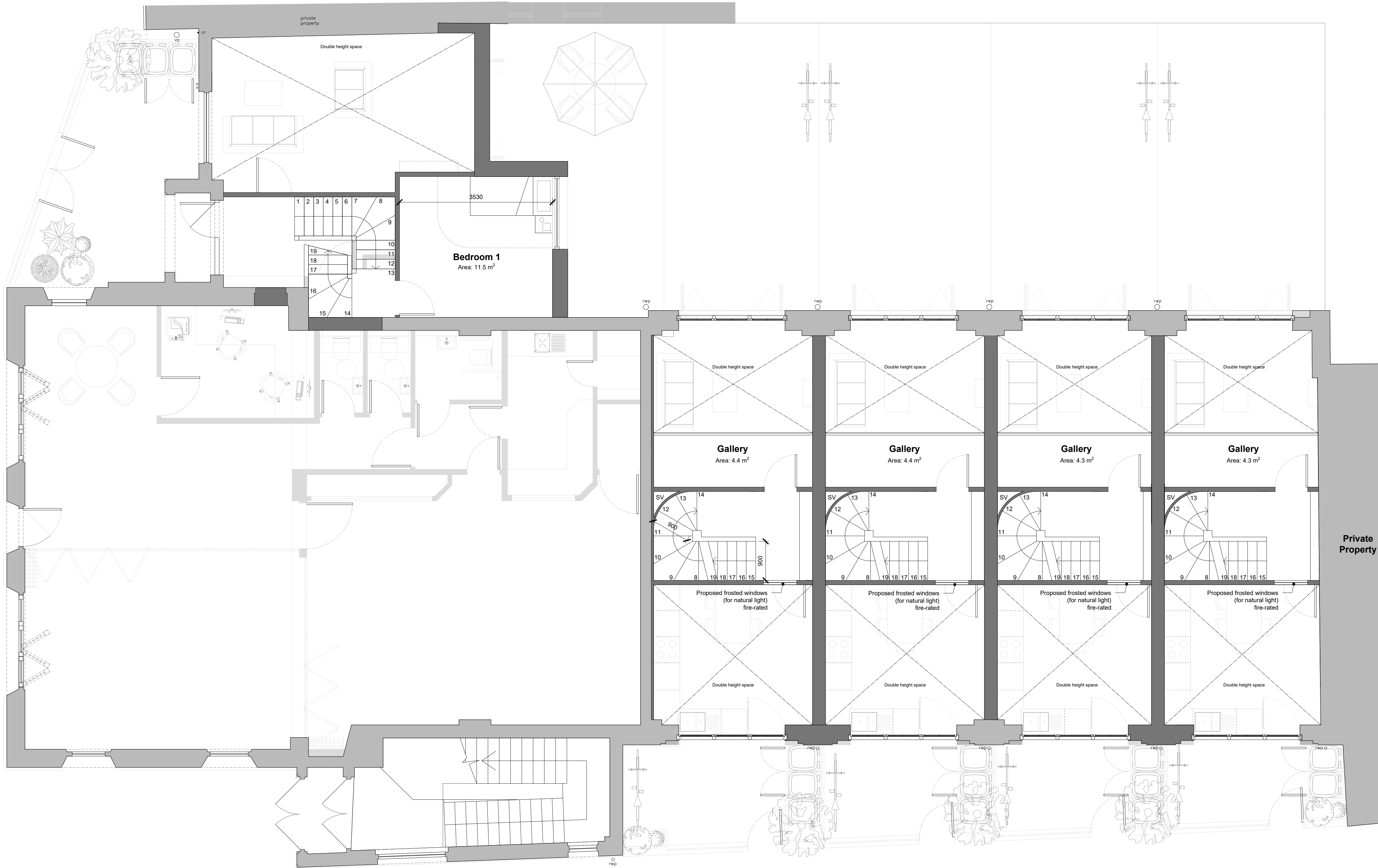
1 Proposed 1:50 Lower First Floor Plan 0 0.5 1.0 2.0 3.0 4.0 5.0 Scale in metres
