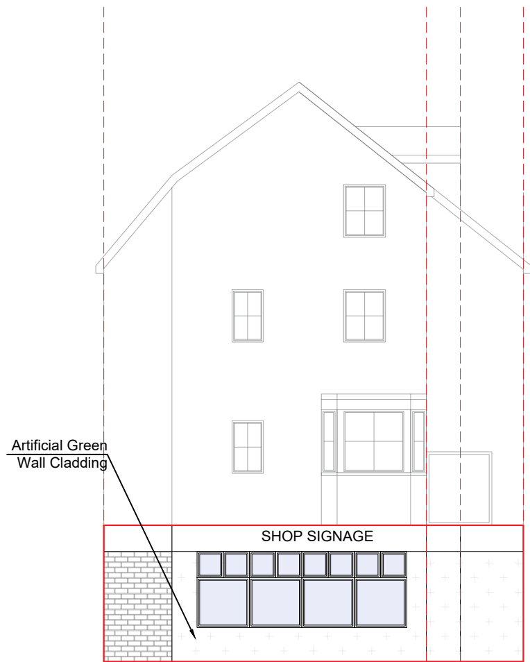
Pre Existing West Elevation
